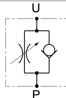
Schema idraulico Hydraulic scheme
